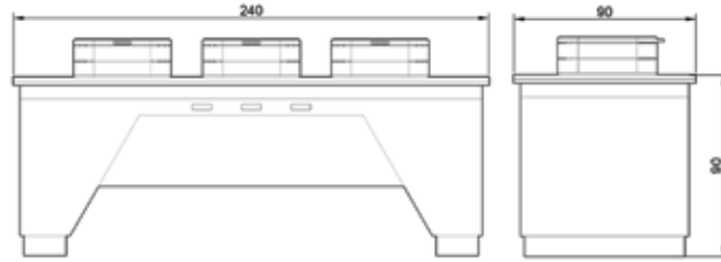
3'LÜ SICAK SERVİS ÜNİTESİ 2400X900X900 TRIPLE CHAFING DISH UNIT 2400X900X900
