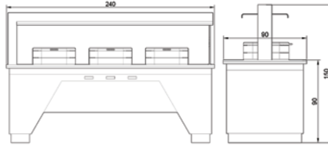
3'LÜ SICAK SERVİS ÜNİTESİ Ö. PERDELİ 2400X900X900/1500 TRIPLE CHAFING DISH UNIT 2400X900X900/1500
